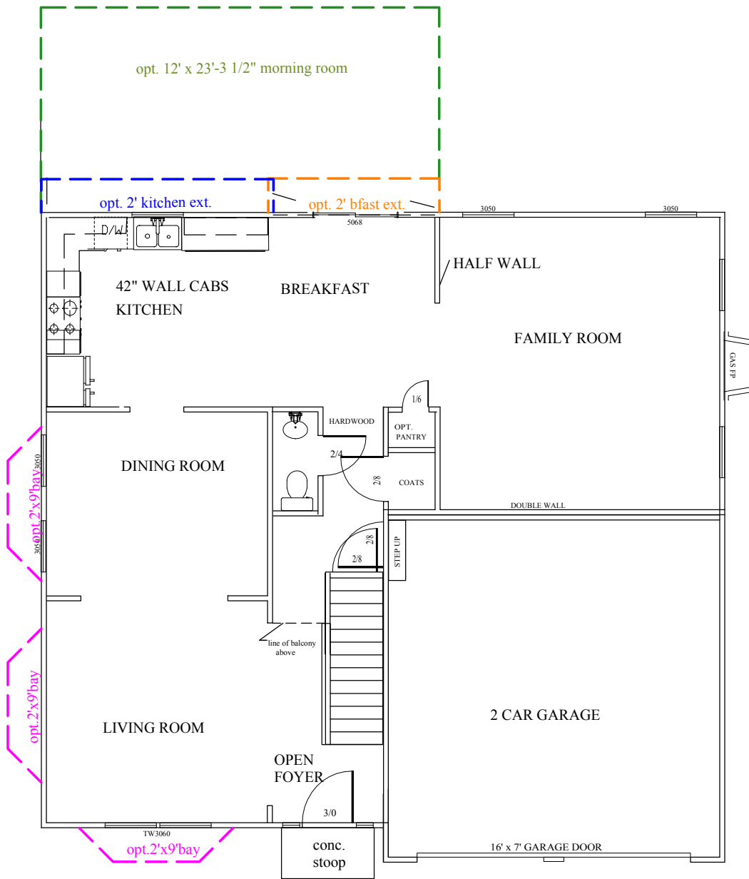
The Rockburne 40 40' first floor plan w/opt.ext.'s&bays
